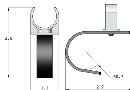
Figure 4. Q035-PIPE
