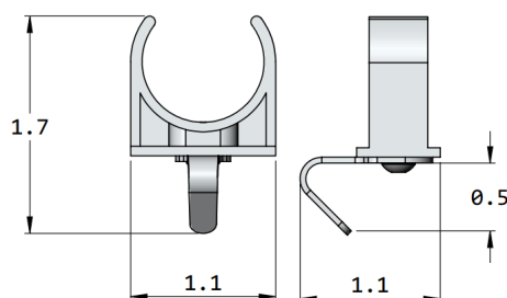
Figure 3. Q035-HOOK
